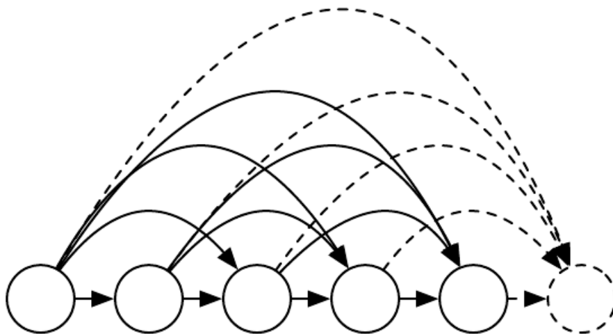
Figure 10.7: Fully connected graphical model for a sequence y^{(1)}, y^{(2)}, \dots, y^{(t)}, \dots, y^{(\tau)} : every past observation y^{(i)} may influence the conditional distribution of some y^{(t)} (for t > i ), given the previous values. Parametrizing the graphical model directly according to this graph (as in Eq. 10.6) might be very inefficient, with an ever growing number of inputs and parameters for each element of the sequence. RNNs obtain the same full connectivity but efficient parametrization, as illustrated in Fig. 10.8.
