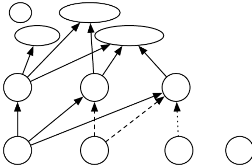
Figure 20.10: An illustration of the neural autoregressive density estimator (NADE). The hidden units are organized in groups \mathbf{h} so that only the inputs x_1, \dots, x_j participate in computing \mathbf{h} and predicting P(x_{j+1} | x_1, \dots, x_j) , for j > i . NADE is differentiated from earlier neural auto-regressive networks by the use of a particular weight sharing pattern: W_{ij} = W_{ik} is shared (indicated in the figure by the use of the same line pattern for every instance of a replicated weight) for all the weights going out from x_i to the k -th unit of any group j \geq i . Recall that the vector (W_{11}, W_{12}, \dots, W_{1n}) is denoted \mathbf{W}_1 .
